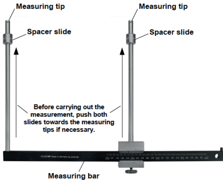
Fig. 1 Product Diagram
