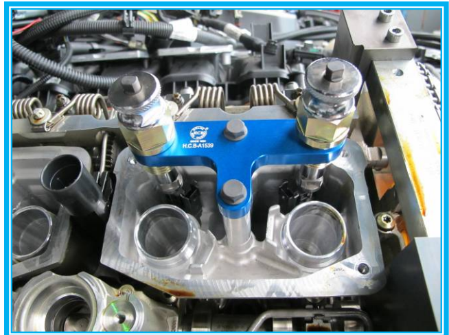
ET1539A use for BMW N20/N55(New Model)
