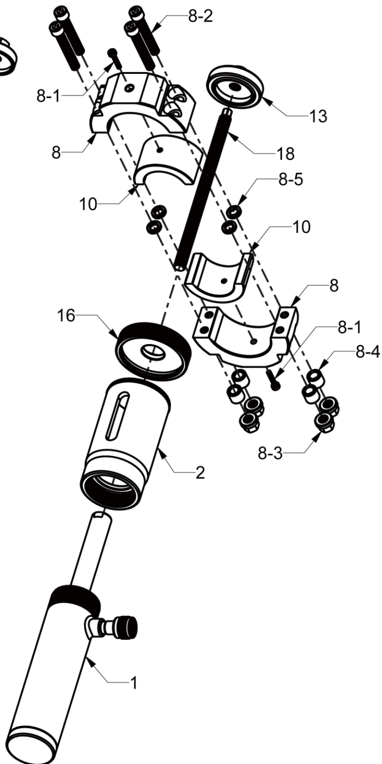
Assembly drawing
