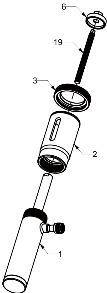
Removal drawing
