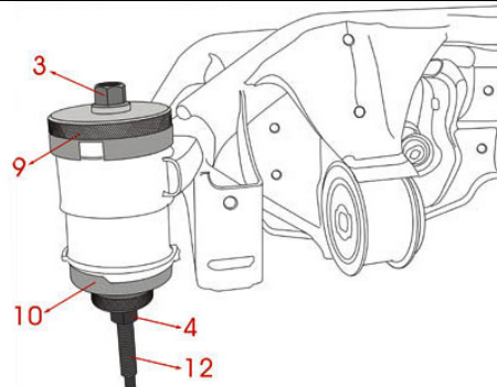
the illustration for installation of rear bush
