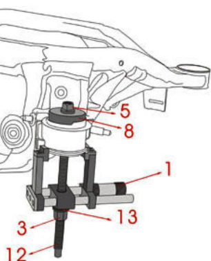
the illustration for installation of F/L bush
