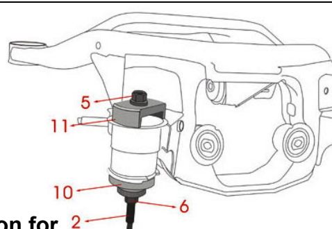
the illustration for installation of F/R bush
