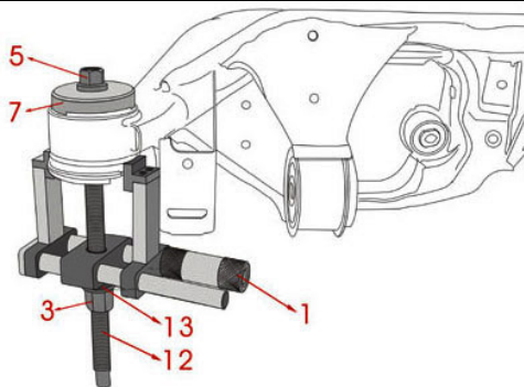
the illustration for removal of rear bush
