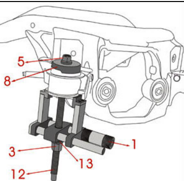
the illustration for removal of F/R bush
